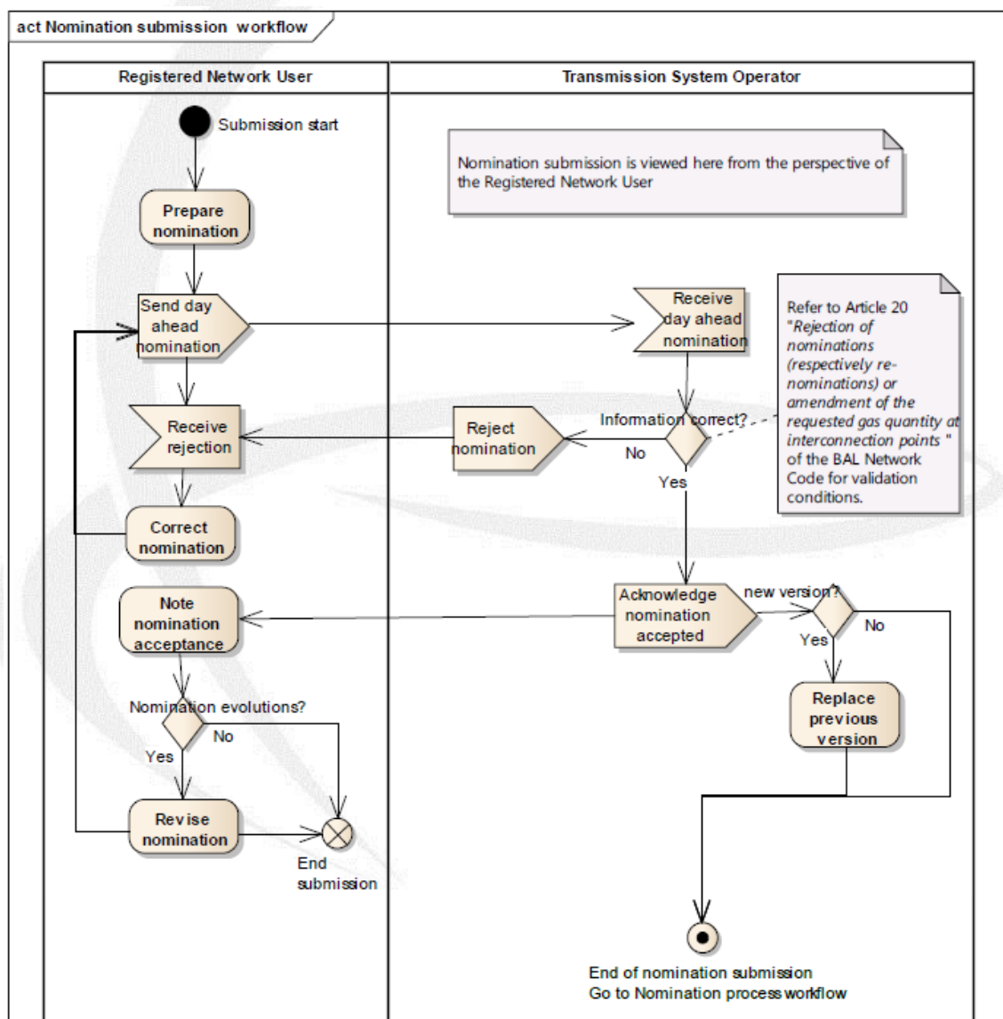
Figure 4: Nomination workflow
